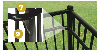
Inside Corner Mount & 90° Elbow Detail
